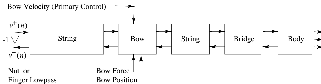
Figure 19. A schematic model for bowed-string instruments.
