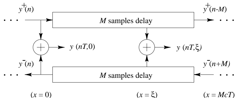
Figure 4. Simplified picture of ideal waveguide simulation.
