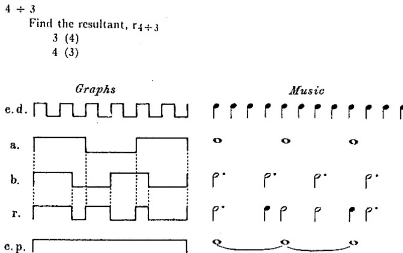
Figure 1 - 4:3 interference pattern
