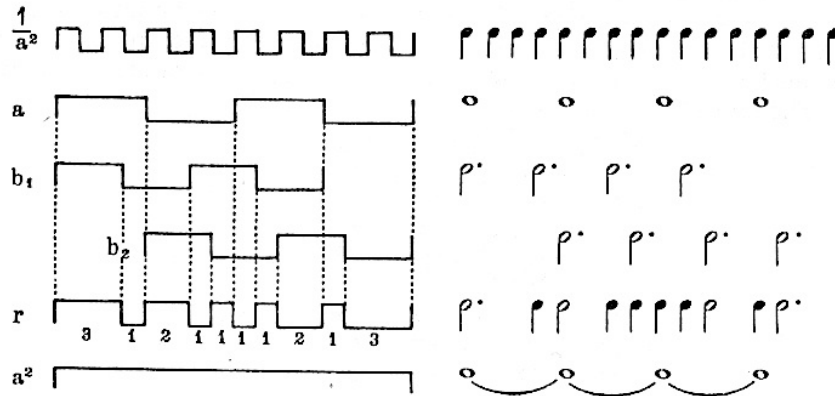
Figure 2 - 2:3 with fractioning
